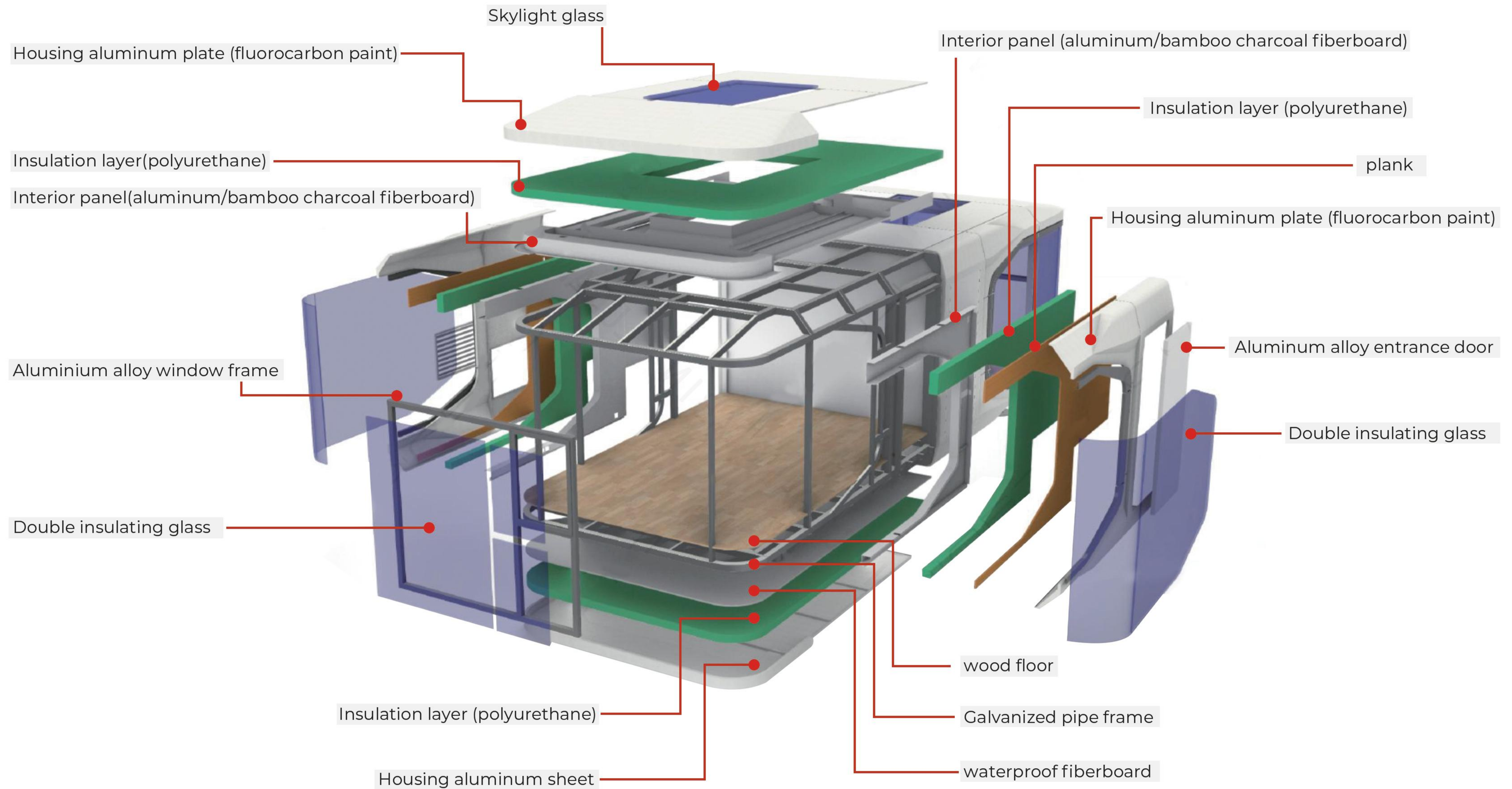
Product Internal Structure Diagram
